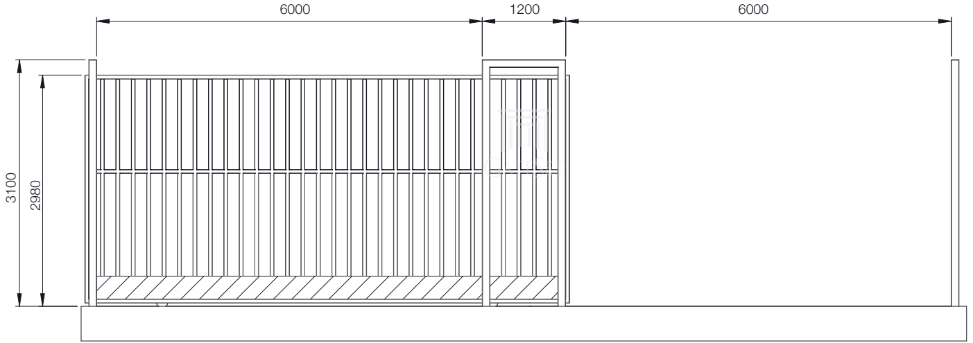
Front View
